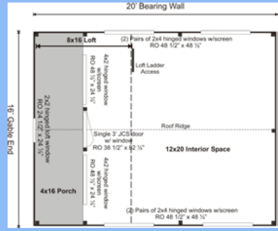
Option C Gable Porch
